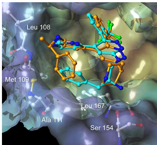
Figure 1. Model of 17 and 32 bound in the ATP-binding site of p38 MAP kinase.
