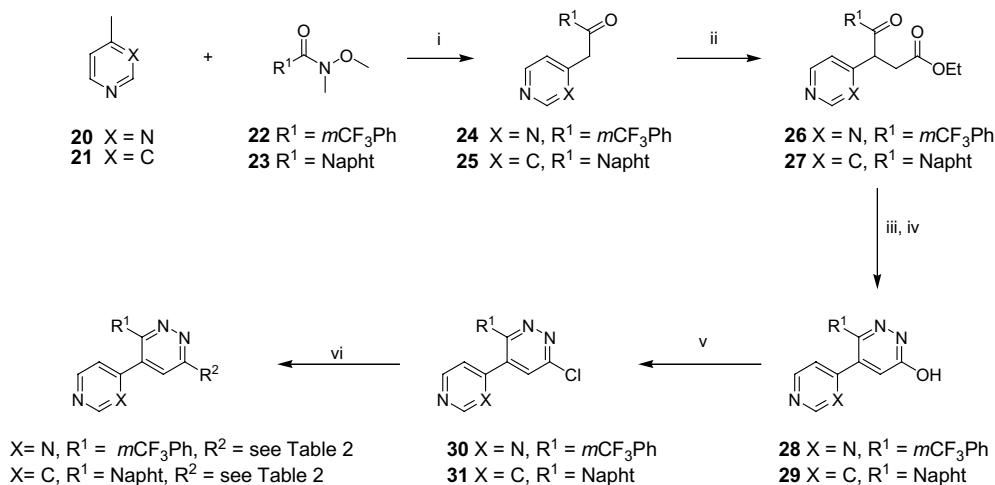
Scheme 2. Synthesis of aminopyridazines. Reagents and conditions: (i) LDA, THF, -78^{\circ}\text{C} , 69–72%; (ii) 60% NaH, DMSO, 0^{\circ}\text{C} , 45 min then ethyl bromoacetate, rt, 18 h, 20%; (iii) \text{N}_2\text{H}_4 , t -BuOH, reflux, 0.5 h, then neat 180^{\circ}\text{C} under high vacuum, quant; (iv) \text{Br}_2 , AcOH, 95^{\circ}\text{C} , 2 h, 51–63%; (v) \text{POCl}_3 , \text{Et}_3\text{BzNCl} , i\text{Pr}_2\text{EtN} , 100^{\circ}\text{C} , 2 h, 58–76%; (vi) \text{R}^2\text{NH} , \text{K}_2\text{CO}_3 , NMP, 100^{\circ}\text{C} , 18 h, 10–35%.
