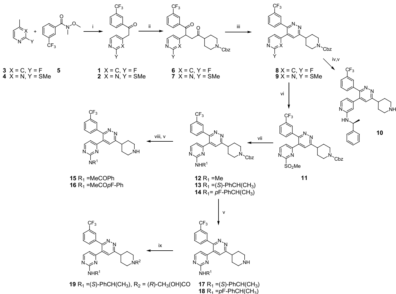
Scheme 1. Synthesis of piperidine-pyridazines. Reagents and conditions: (i) LDA, THF, -78^{\circ}\text{C} , 60–64%; (ii) 60% NaH, DMSO, rt, 0.5 h then 4-(2-chloroacetyl)-piperidine-1-carboxylic acid benzyl ester, rt, 18 h, 26–28%; (iii) (a) \text{N}_2\text{H}_4 , t -BuOH, reflux, 0.5 h, then neat heated at 180^{\circ}\text{C} under high vacuum; (b) DDQ, toluene, rt, 18 h, 32–75%; (iv) ( S )- \alpha -methylbenzylamine, 125^{\circ}\text{C} , 3 h, 70%; (v) Pd/C, \text{H}_2 , rt, 18 h, 31–87%; (vi) 30% \text{H}_2\text{O}_2 , \text{Na}_2\text{WO}_4 \cdot 2\text{H}_2\text{O} , MeOH, reflux, 18 h, 90%; (vii) \text{R}^1\text{NH}_2 neat 125^{\circ}\text{C} , 57–70%; (viii) \text{ArCOCl} , \text{Et}_3\text{N} , DCM, rt, 88–95%; (ix) EDC, HOBT, ( R )-lactic acid, 93%.
