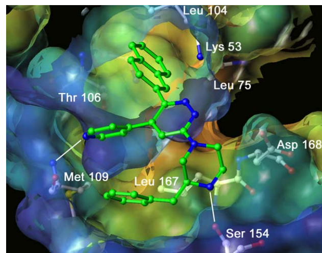
Figure 2. X-ray crystal structure of 39 cocrystallized with p38 MAP kinase.
